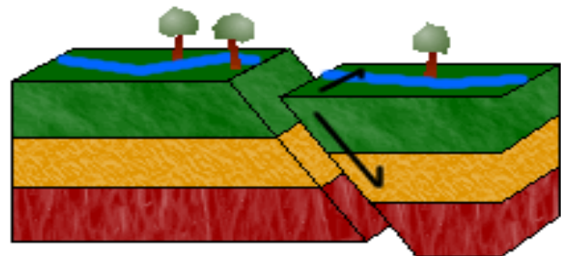
Oblique-slip
